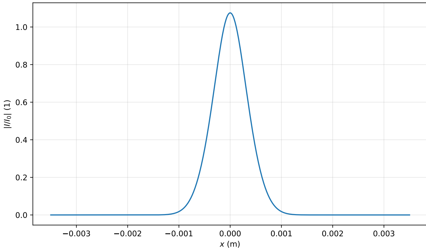
Intensity profile I(x, y = 0, z = 0.318m)/I_0 , P_{in}=1.0P_{cr} , artificial time
